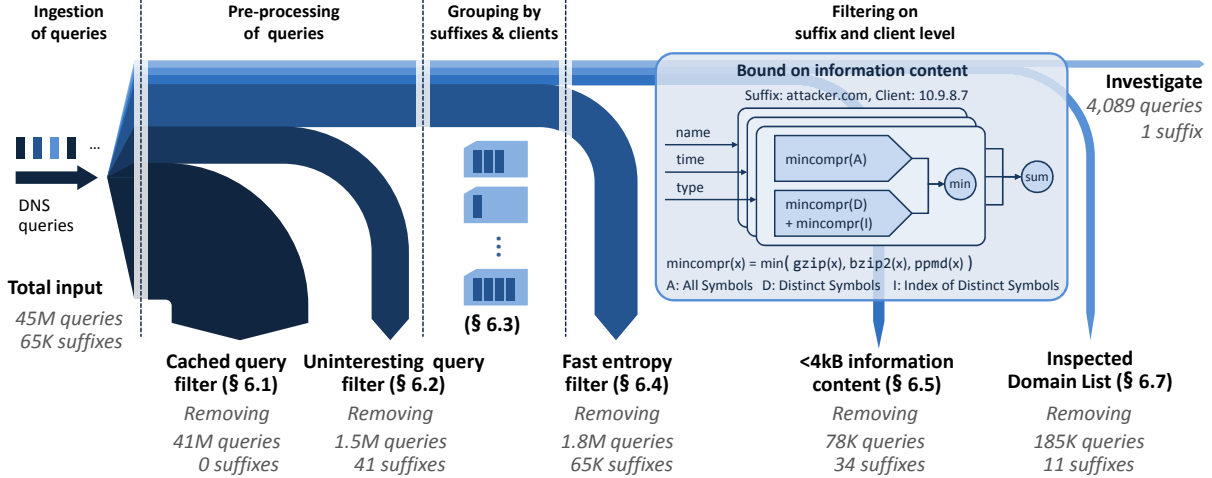
Figure 5: The full detection procedure. The numbers (grey) reflect a day at the INDLAB network for which the detection procedure flagged a new domain name (a relatively rare event).
