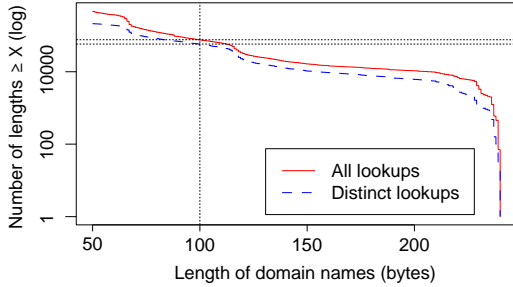
Figure 3: Distribution of the lengths of all individual (solid) or all distinct (dashed) domain name prefixes queried during a sample day of data from LBL. The horizontal lines mark that 76K (all) and 58K (distinct) lookups were \geq 100 bytes. Lengths do not include the registered domain targeted by the lookup. Note that the plot shows the upper 1% of all queries, but the upper 18% of all distinct queries.
